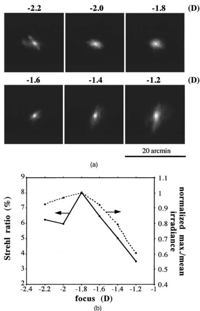
Fig. 4. (a) Double-pass aerial images for observer CG in different foci when using green light and 4-mm pupil diameter in both passes. (b) Two different image-quality criteria used to select the best image: the Strehl ratio (solid curve) and the normalized maximum divided by the mean irradiance (dotted curve) as a function of focus.
