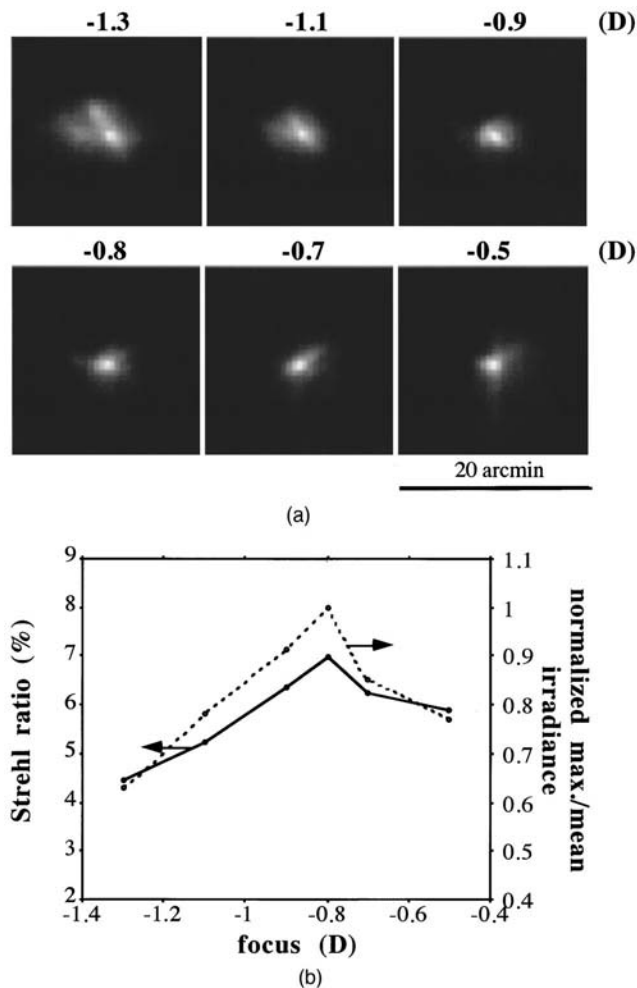
Fig. 5. (a) Double-pass aerial images for observer CG in different foci with near-infrared light and 4-mm pupil diameter in both passes. (b) Two different image-quality criteria used to select the best image: the Strehl ratio (solid curve) and the normalized maximum divided by the mean irradiance (dashed curve) as a function of focus.
