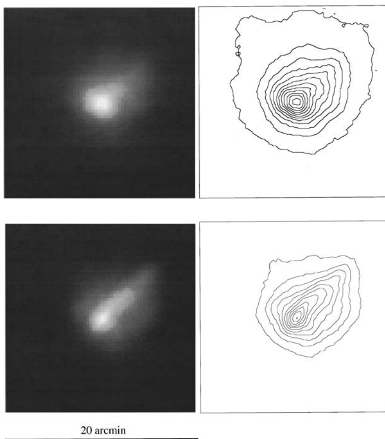
Fig. 11. Gray-level and contour plots for near-infrared (top) and green (bottom) retinal images recorded with unequal first- (1.5-mm) and second-pass (6-mm) stops for subject NL. These double-pass images contain information on ocular asymmetric aberrations. Note that the two images have roughly the same shape.
