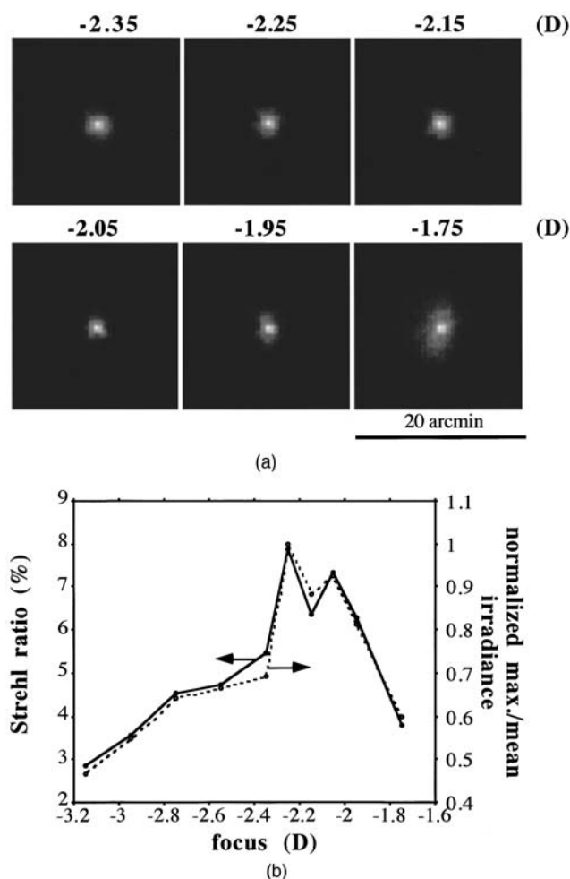
Fig. 2. (a) Double-pass aerial images for observer PA in different foci with green light and 4-mm pupil diameter in both passes. (b) Two different image-quality criteria used to select the best image: the Strehl ratio (solid curve) and the normalized maximum divided by the mean irradiance (dashed curve) as a function of focus.
