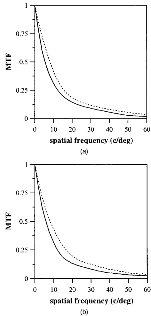
Fig. 9. MTF's calculated from double-pass images for subjects (a) NL and (b) PA with near-infrared (solid curves) and green (dashed curves) light when 4-mm pupil diameter was used.
