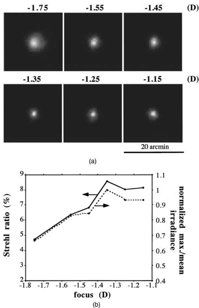
Fig. 3. (a) Double-pass aerial images for observer PA in different foci with near-infrared light and 4-mm pupil diameter in both passes. (b) Two different image-quality criteria used to select the best image: the Strehl ratio (solid curve) and the normalized maximum divided by the mean irradiance (dashed curve) as a function of focus.
