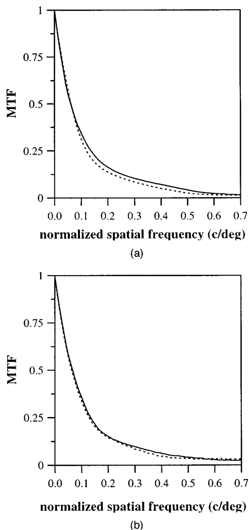
Fig. 10. Same MTF results as in Fig. 9 represented versus the normalized spatial frequency (divided by the cutoff spatial frequency for the diffraction-limited case). Solid and dashed curves correspond to near-infrared and green light, respectively.
